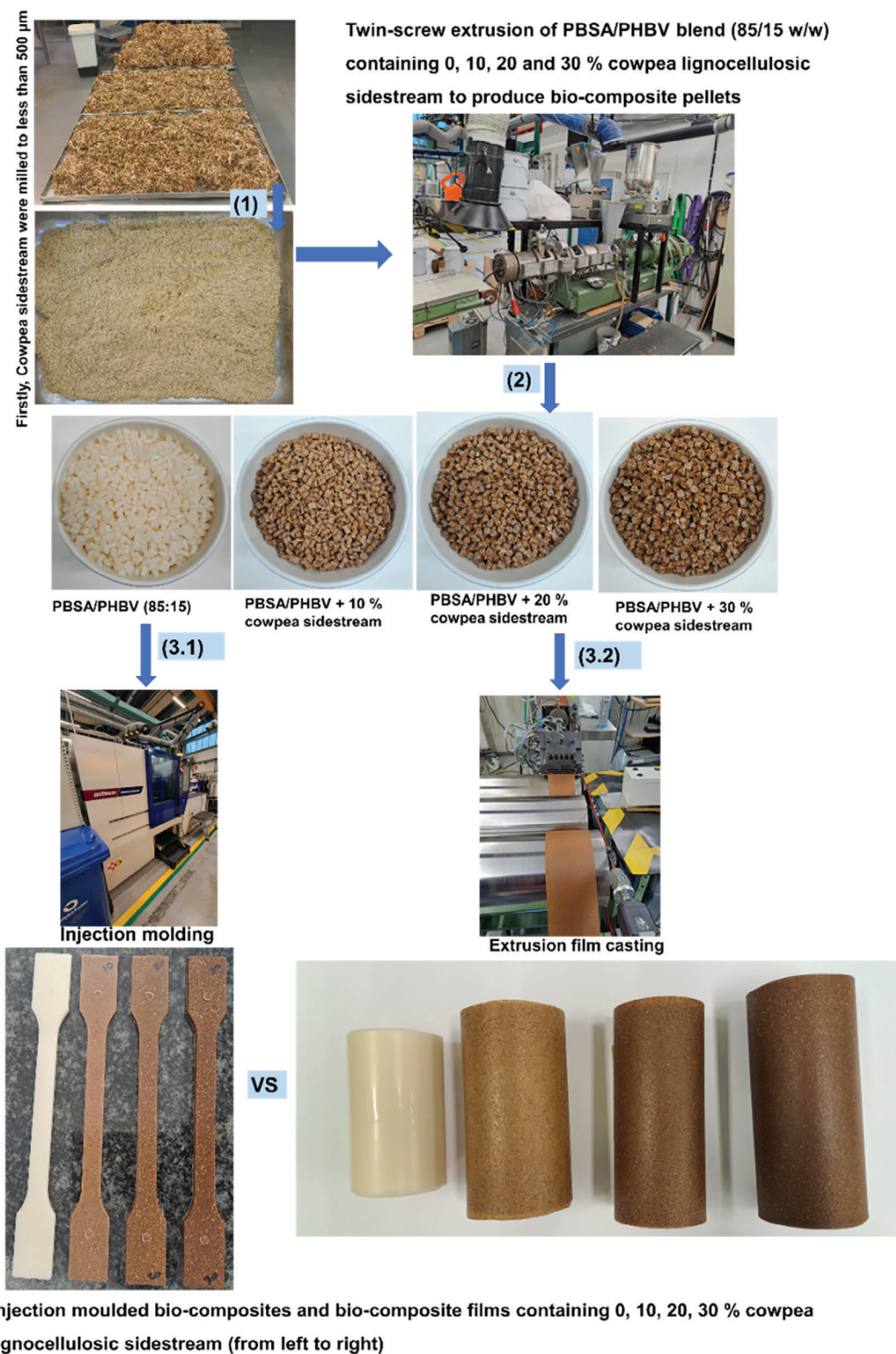
Figure 1. Processing steps to produce injection molded bio-composites and bio-composite films containing 0, 10%, 20%, and 30% cowpea lignocellulosic sidestream. Step 1 shows the milled cowpea sidestream, step 2 shows the compounding of polymers and fibers to produce bio-composite pellets; step 3.1 shows injection molding, and step 3.2 shows extrusion film casting.
